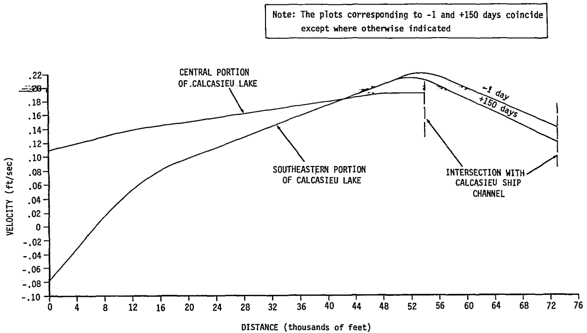
Figure D.13-6. Spatial Variation of Flow Velocity in Calcasieu Lake
