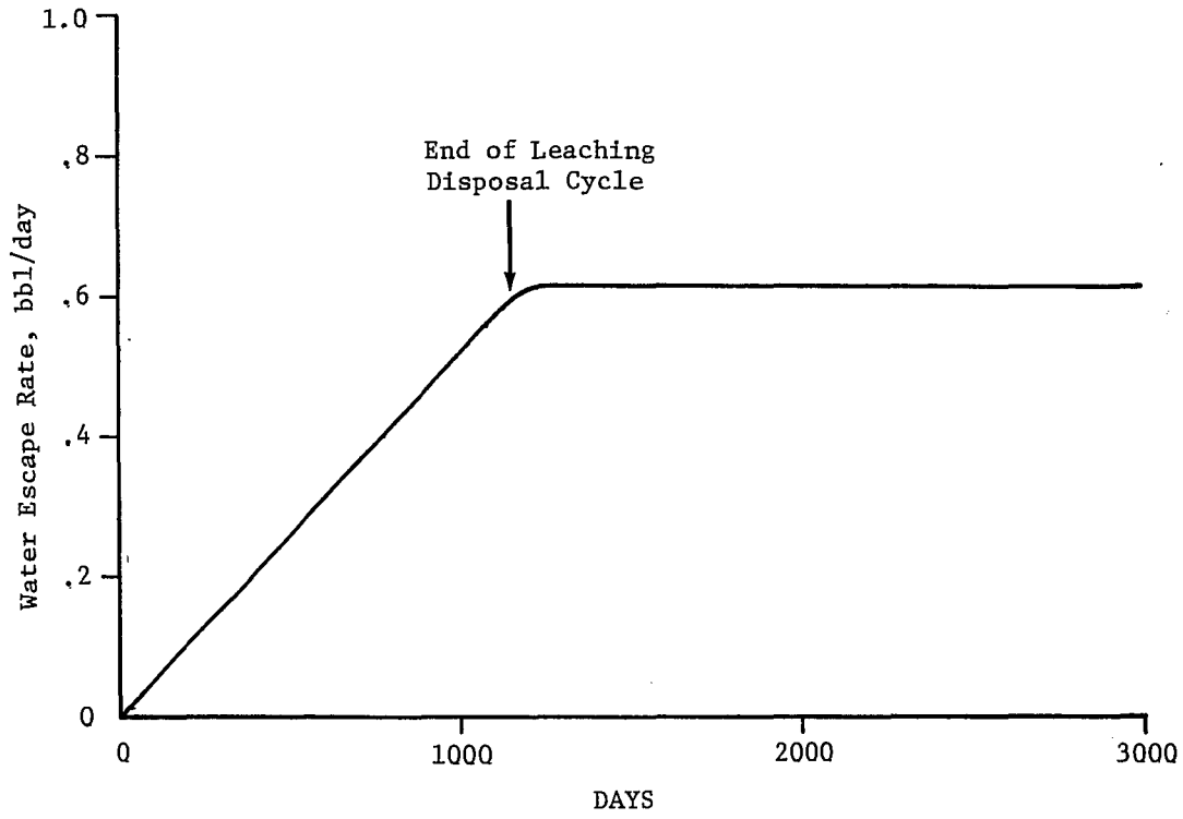
Figure D.23-1 Water Loss Through an Improperly Plugged Abandoned Well
