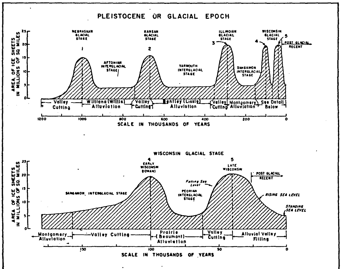
Figure P-3. Pleistocene events of Texas and Louisiana modified after Fisk (1944).
