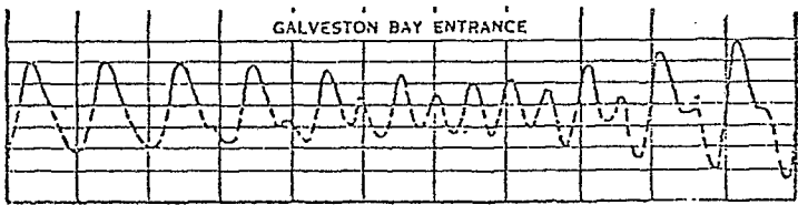
Figure 16. Tidal Currents, Galveston Bay Entrance (Source: Tidal Current Tables, NOAA, 1977).
