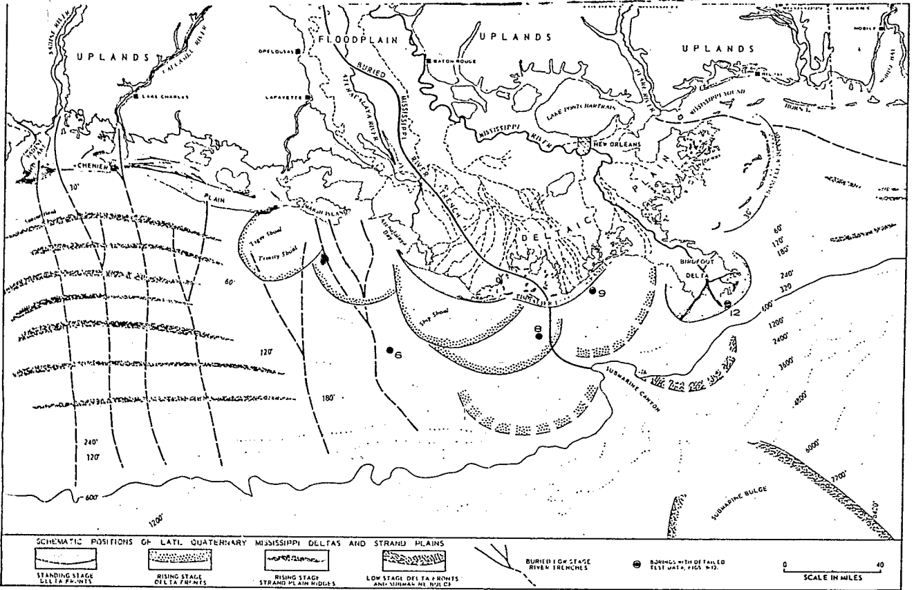
Fig. P-8 Positions of Late Quaternary Buried Trenches, Strand Plains, and Deltas off Louisiana Coast. (Fisk and McLellan, 1959).
