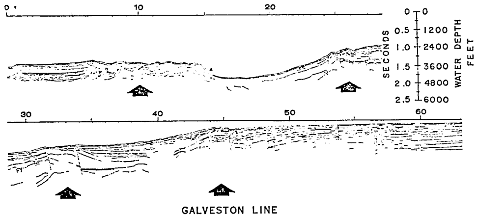
Figure P-5 Line drawing of Electro-Sonic Profiler record of the Galveston line. (Moore and Curray, 1963). Arrows indicate centers of upthrusting.
