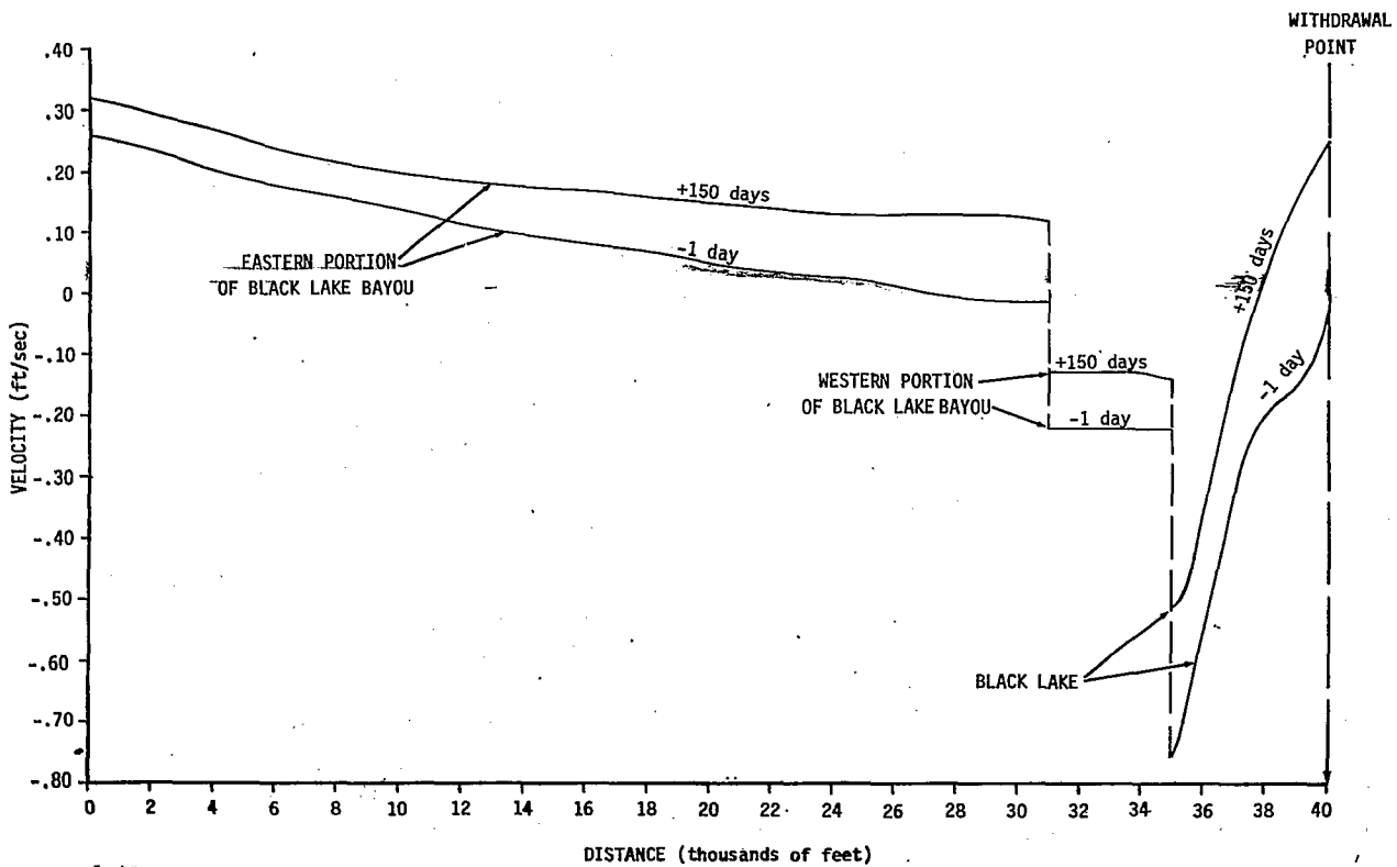
Figure D.12-4. Spatial Variation of Flow Velocity in Black Lake and Black Lake Bayou (Without Wind-Driven Tidal Effects)
