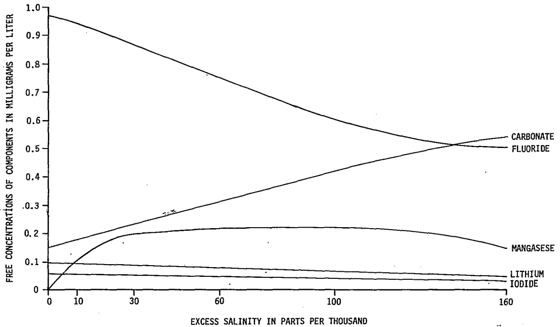
Figure D.15-5. Free (Unbound) Concentrations of Components at Various Salinity Contours
