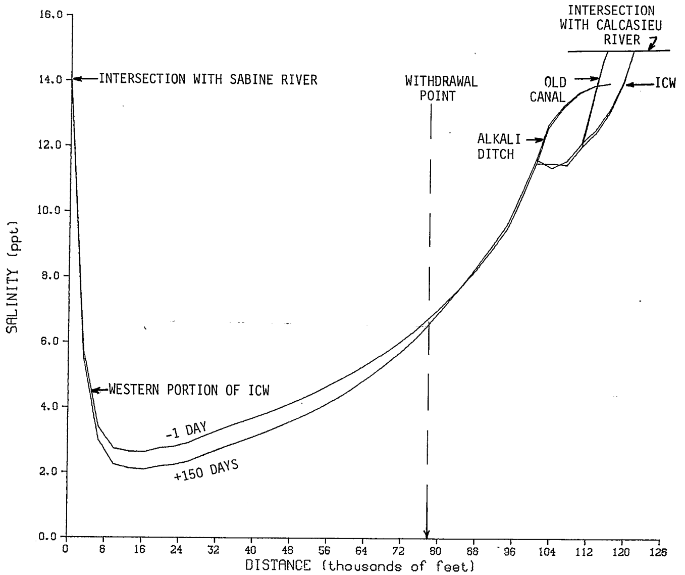
FIGURE D.27-3 SPATIAL VARIATION OF SALINITY IN THE ICW, OLD CANAL AND ALKALI DITCH. (TEST CASE 1- HYDRAULIC BOUNDARY CONDITIONS IN ALKALI DITCH.)
