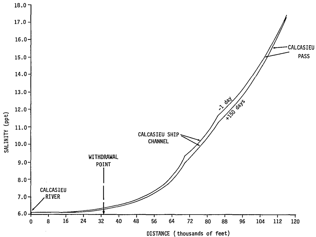
Figure D.13-2. Spatial Variation of Salinity in Calcasieu Ship Channel and Pass
