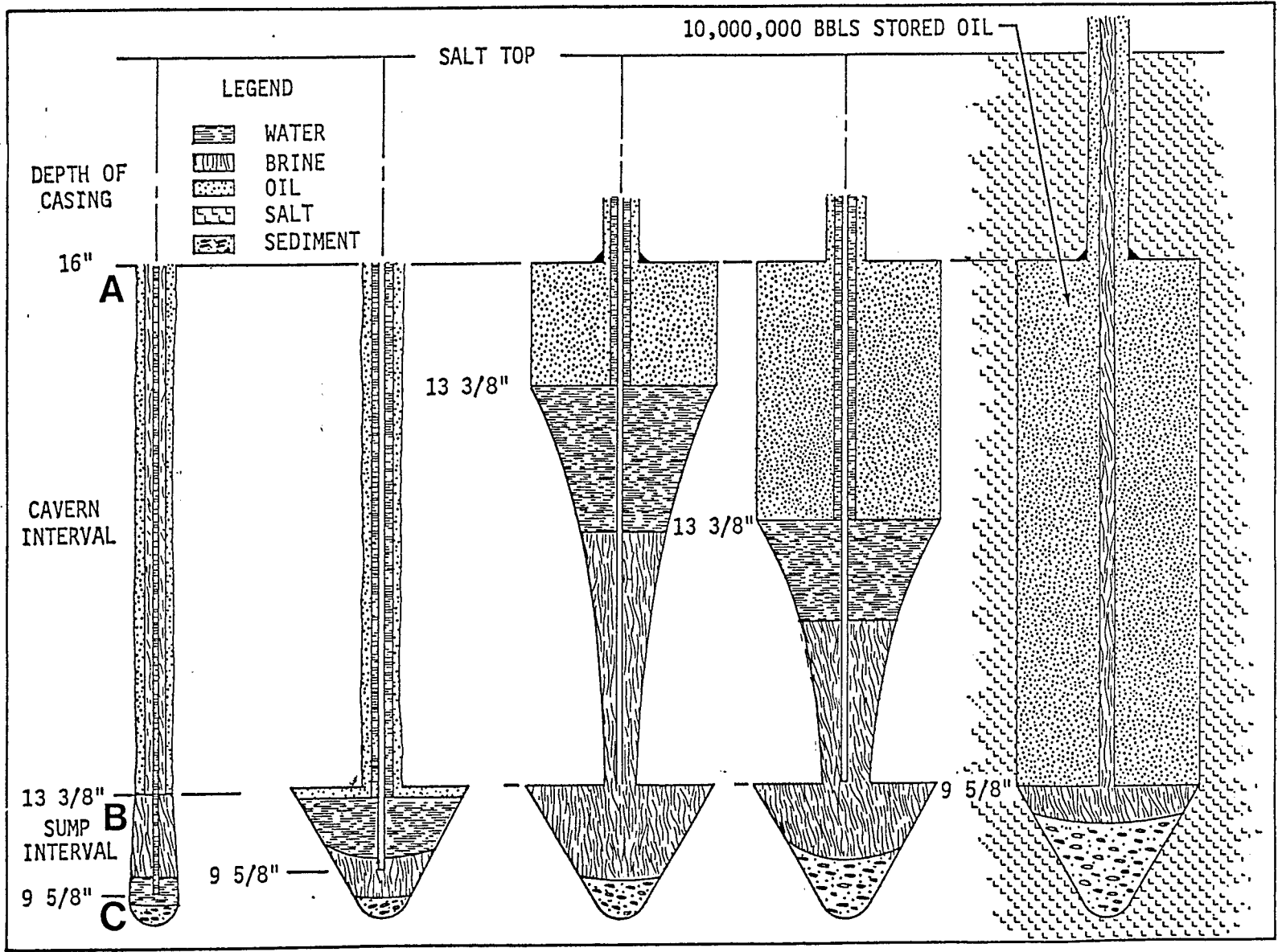
Figure J-3. Concurrent Storage & Leaching Process
