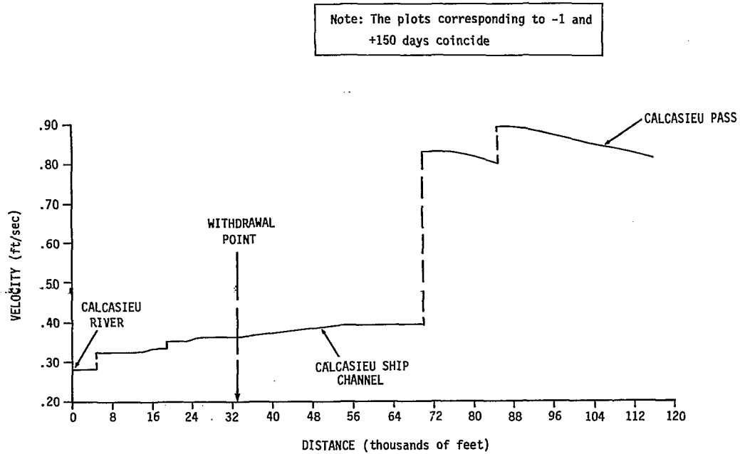
Figure D.13-5. Spatial Variation of Flow Velocity in Calcasieu Ship Channel and Pass
