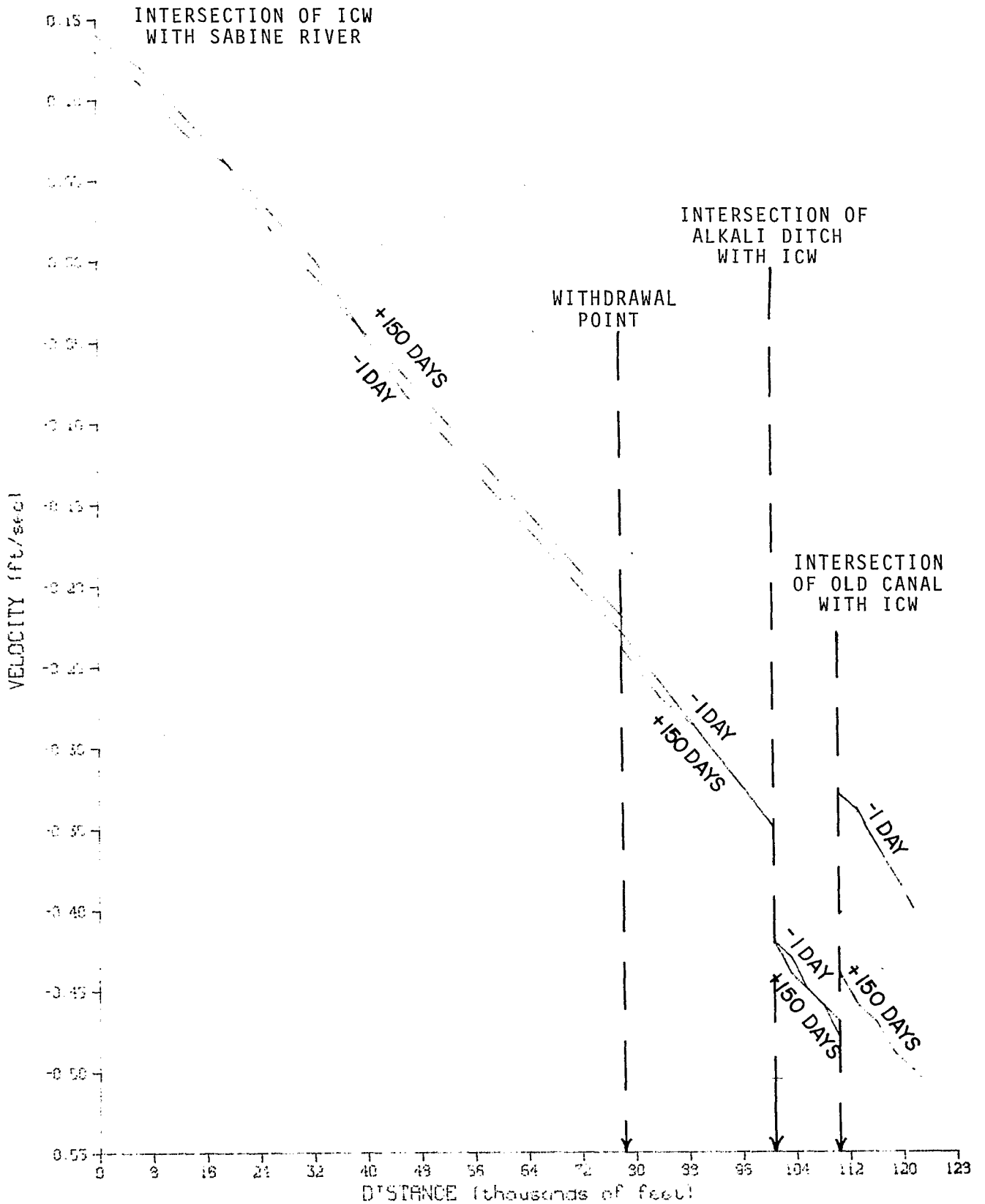
FIGURE D.27-7 SPATIAL VARIATION OF FLOW VELOCITY IN ICW. (TEST CASE 2- NO HYDRAULIC BOUNDARY CONDITIONS IN ALKALI DITCH.)
