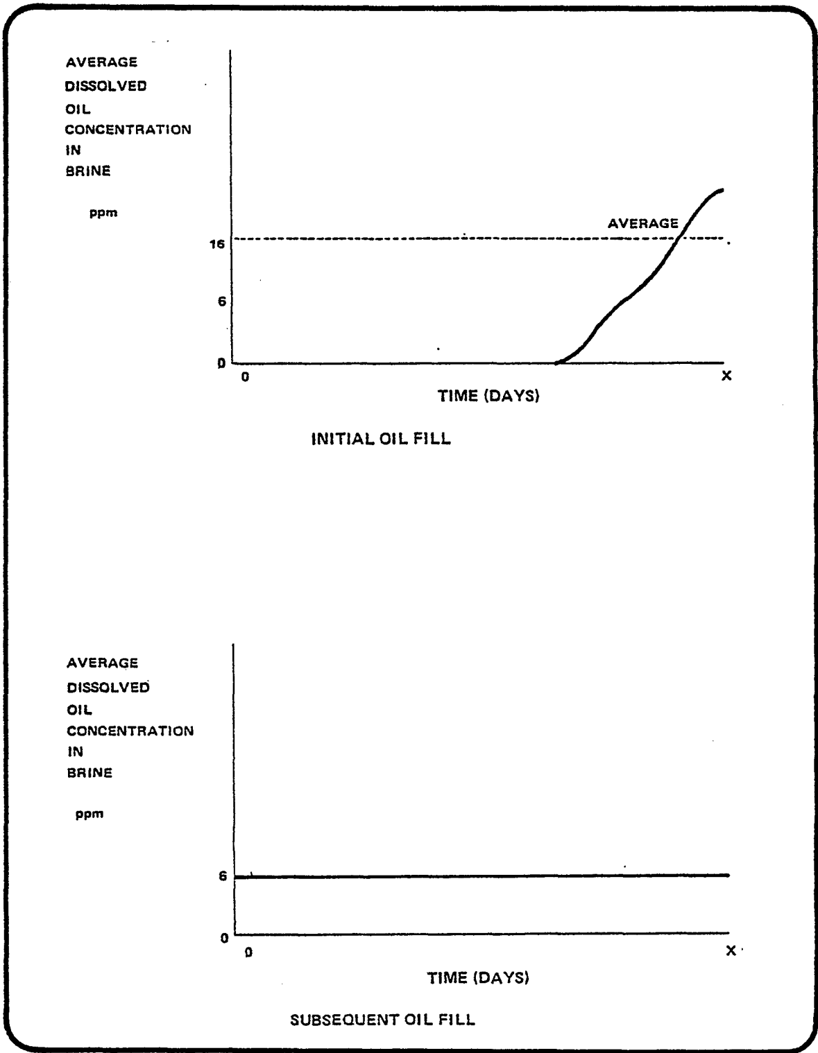
FIGURE S-6 Schematic representation of oil in brine concentrations discharged from a typical cavern
