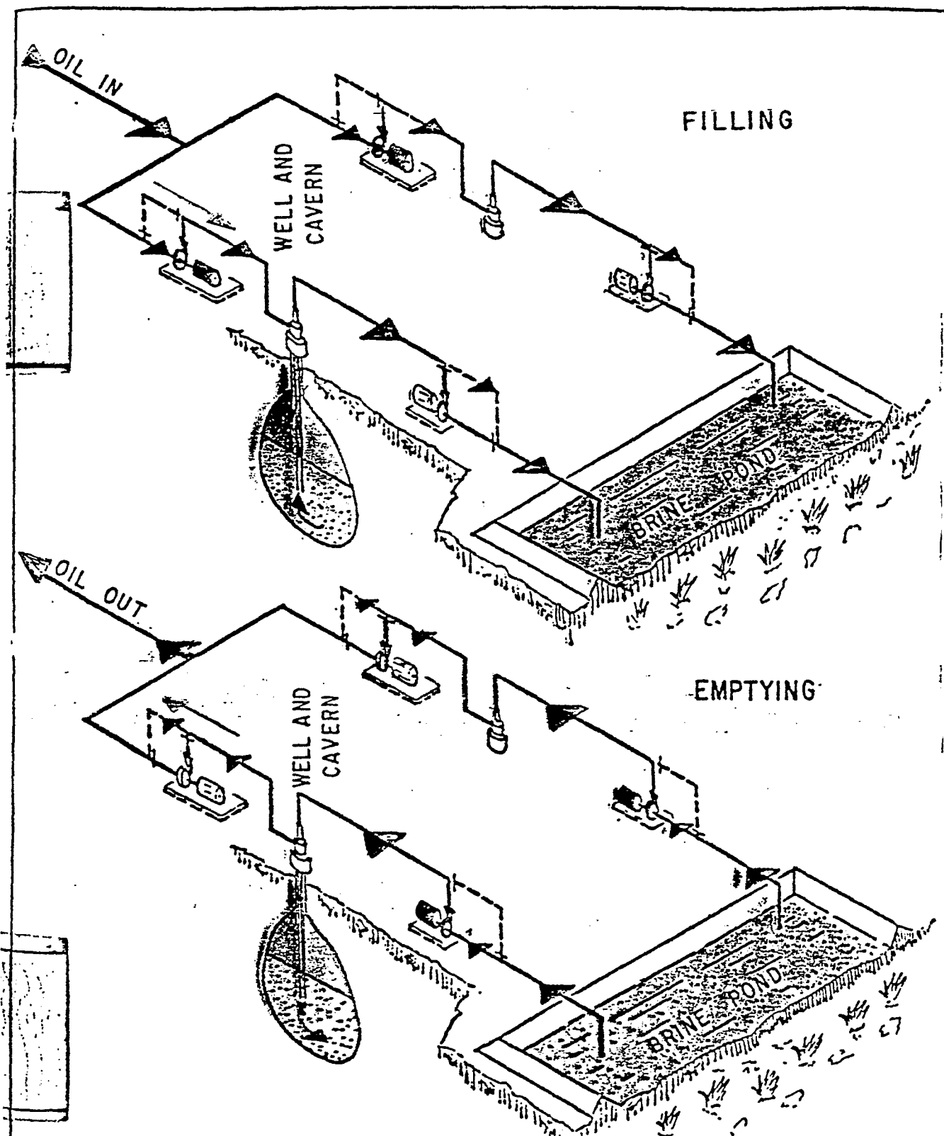
UNDERGROUND STORAGE FOR PETROLEUM PRODUCTS IN LEACHED CAVERN OPERATION PROCESS
