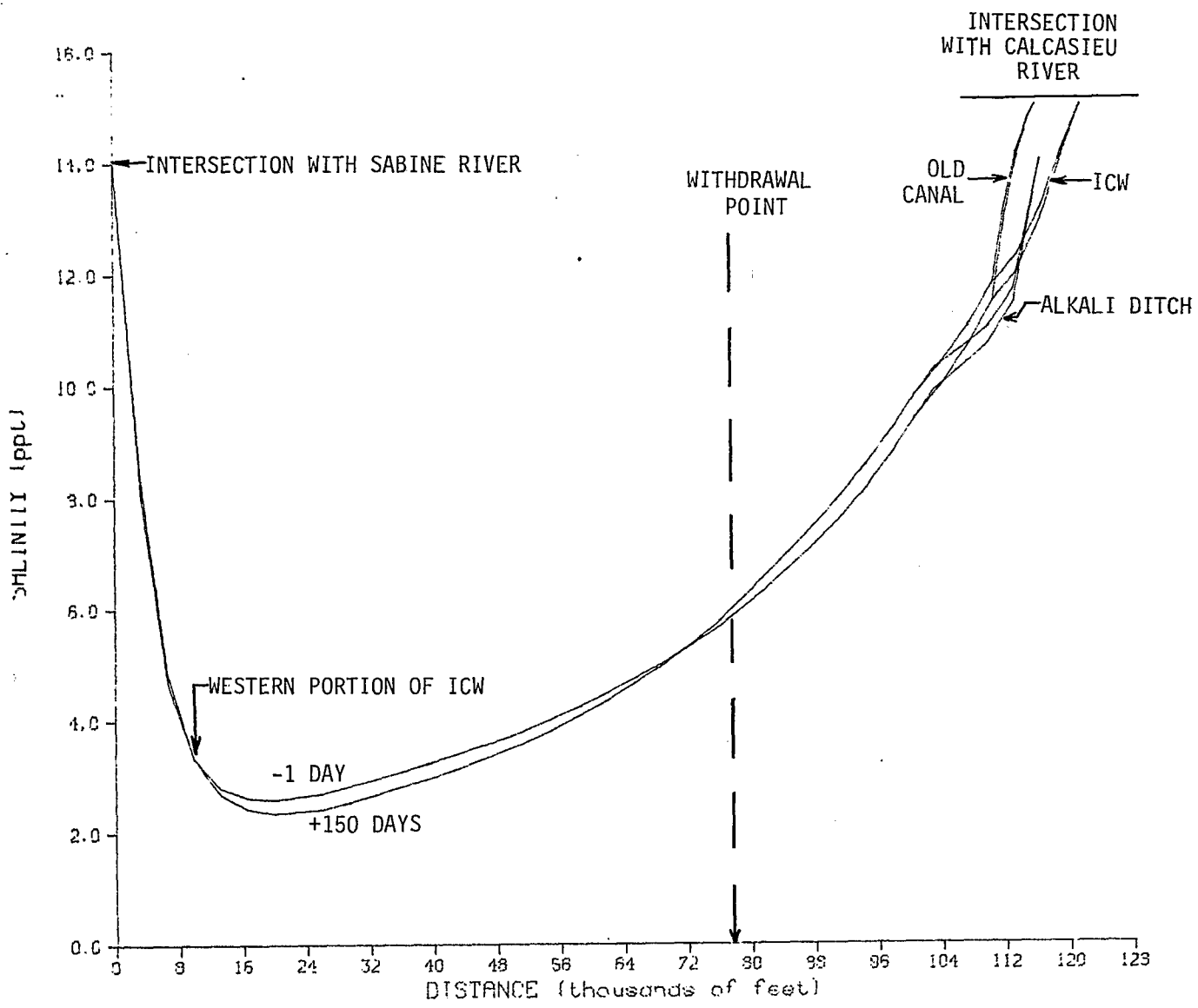
FIGURE D.27-6 SAME AS D.27-3 EXCEPT (TEST CASE 2- NO HYDRAULIC BOUNDARY CONDITION IN ALKALI DITCH.)
