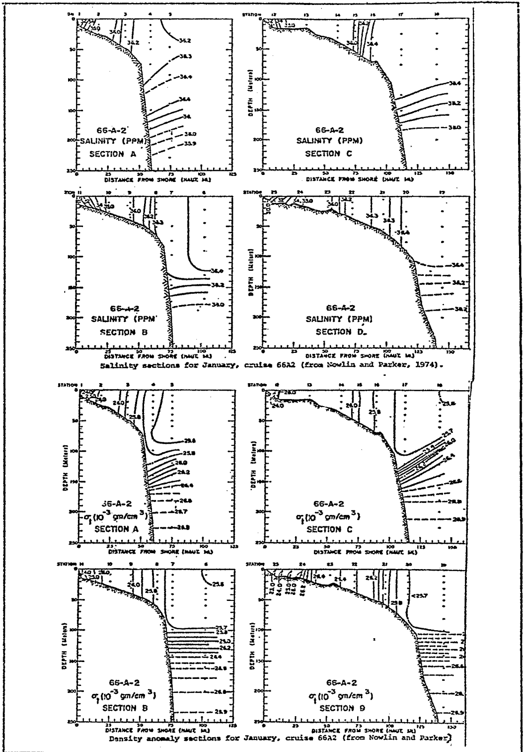
Figure 13 Density Anomaly Sections for January, Cruise 66A2 (Nowlin and Parker, 1974)
