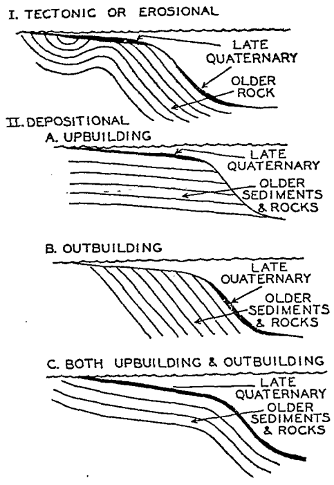
Fig. P-7 Basic descriptive classification of continental terrace structural types. (Moore and Curray, 1963).
