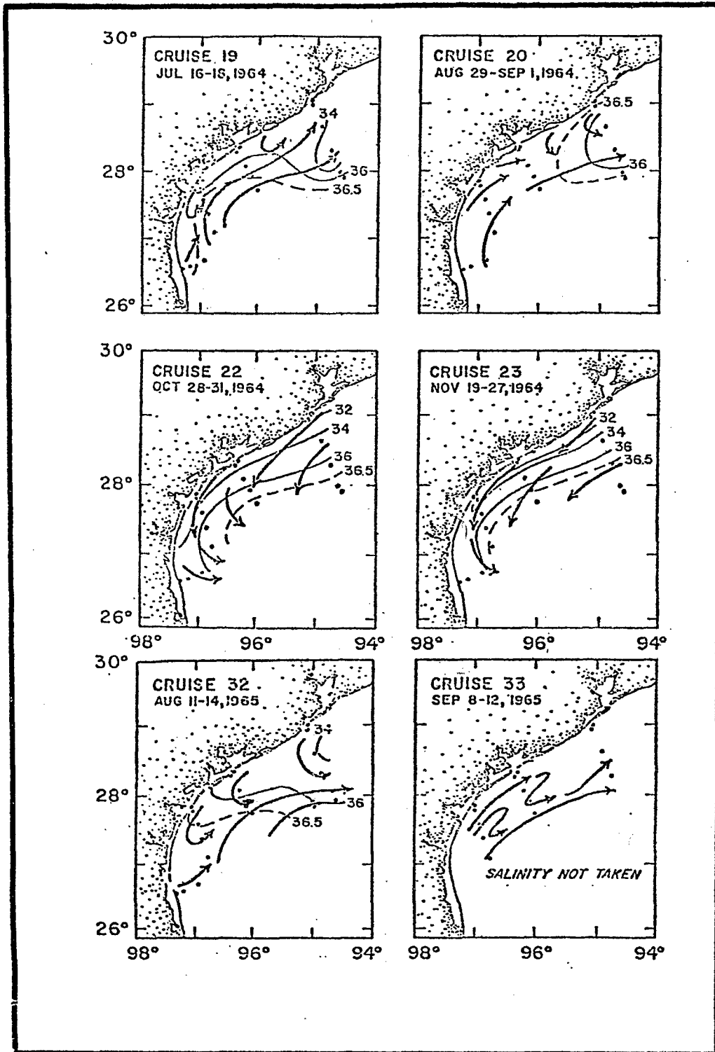
Figure 26 Shelf water circulation and surface salinity ( ^{\circ}/_{\infty} ) GUS III cruises (1963-1965).
