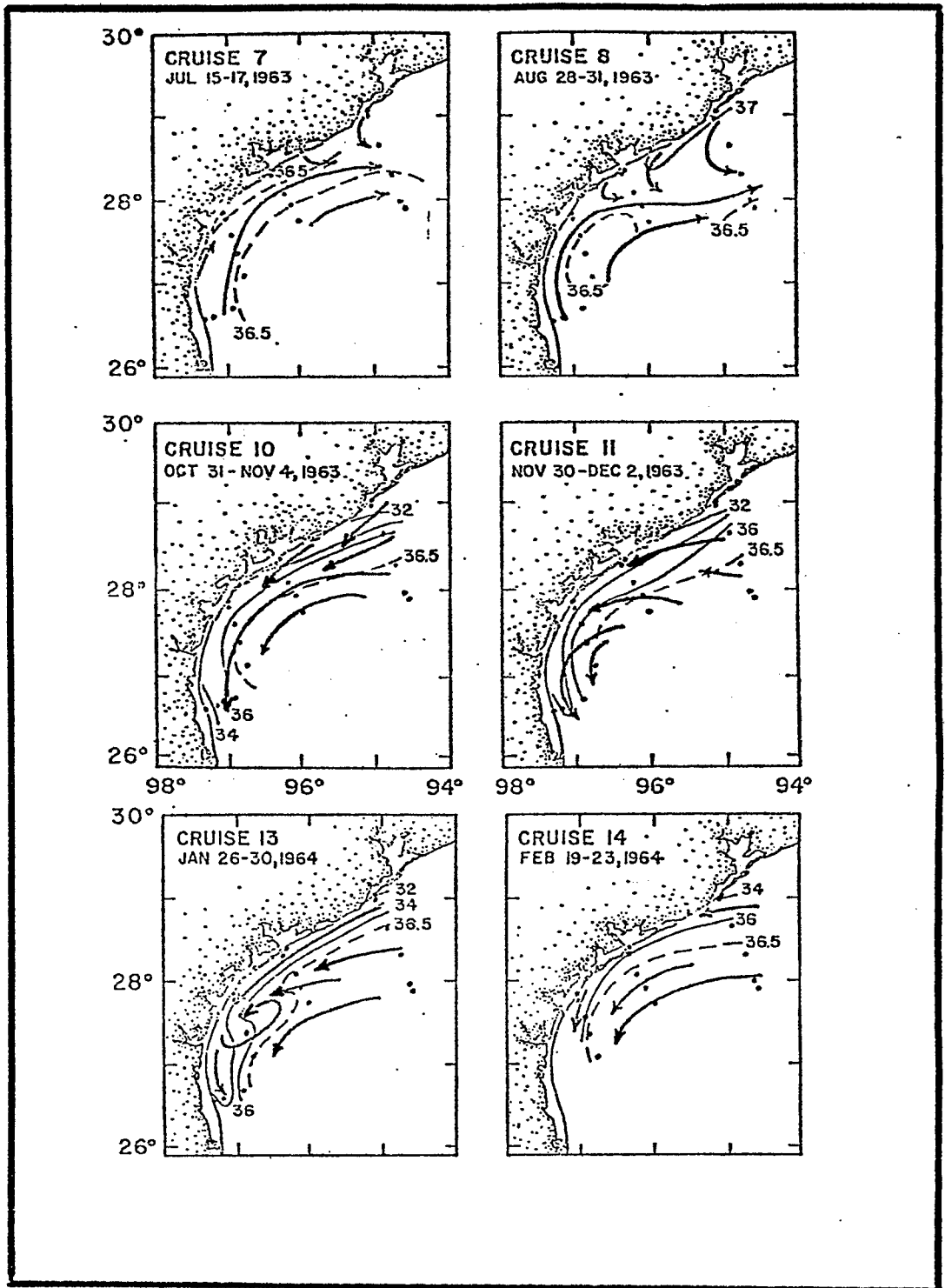
Figure 25 Shelf water circulation and surface salinity ( ^{\circ}/_{00} ) GUS III cruises (1963-1965).
