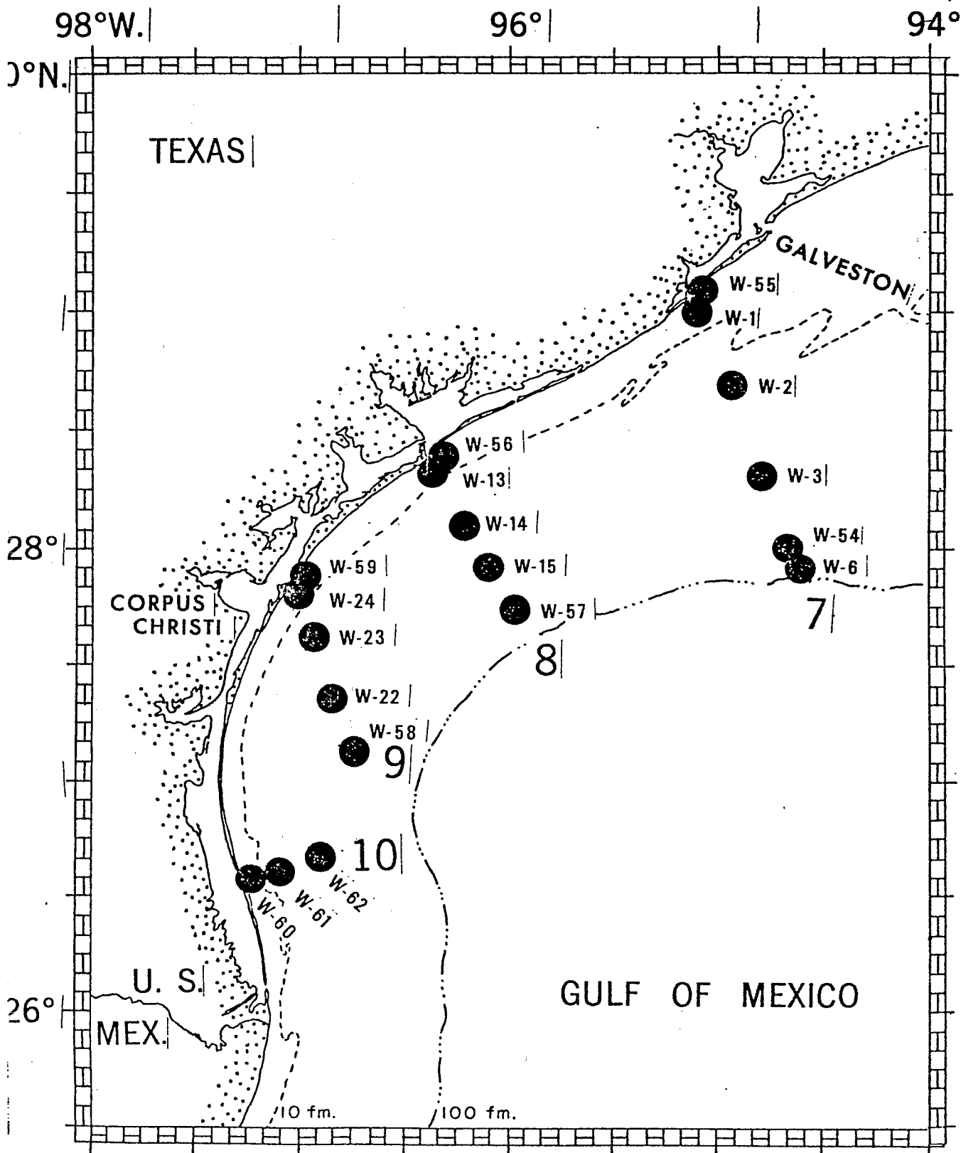
Figure Q-12 The location of transects 7-10 with their respective stations at which monthly sampling was conducted between January 1963 and December 1965.
