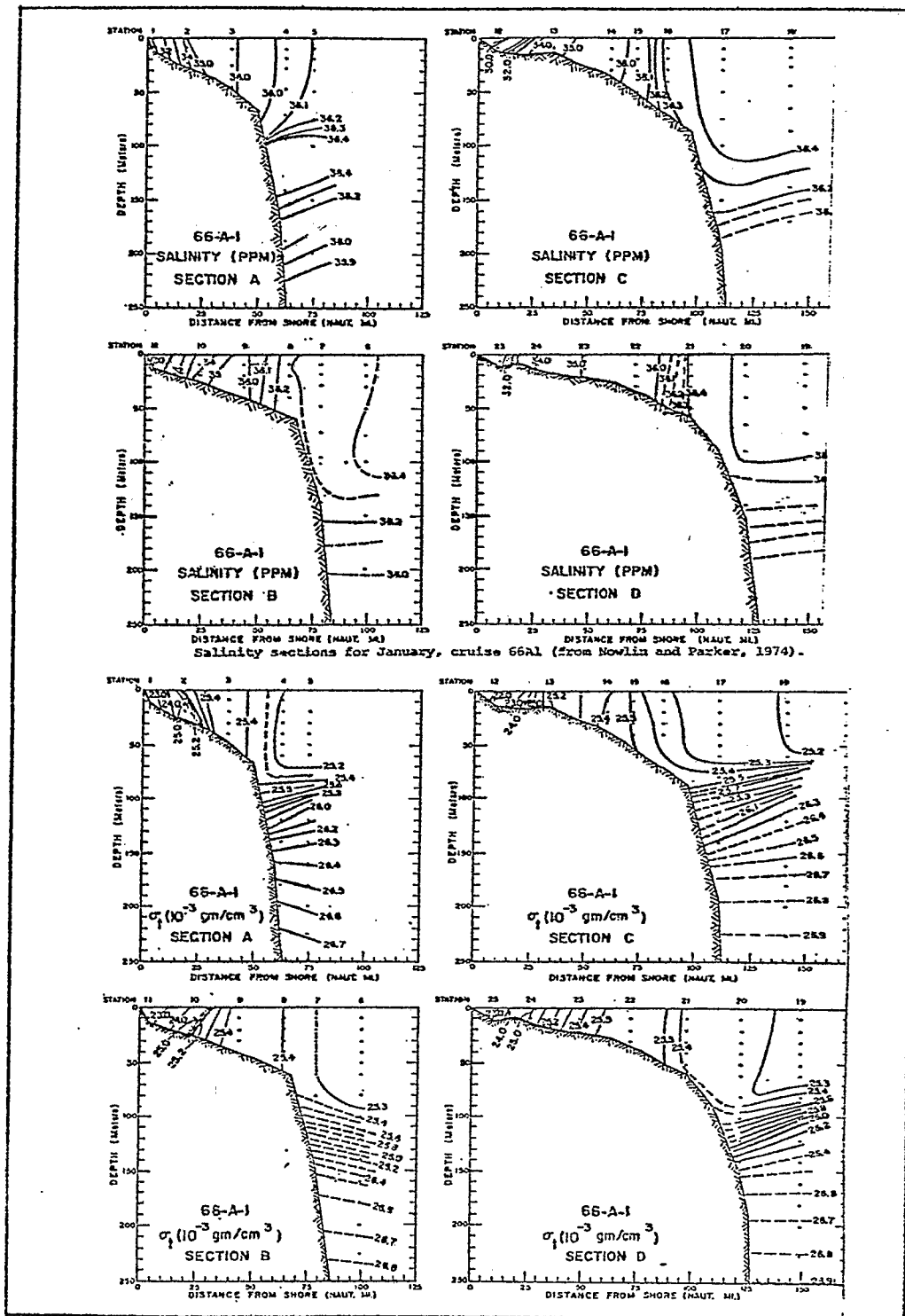
Figure 14 Density Anomaly Sections for January, Cruise 66A1 (Nowlin and Parker, 1974)
