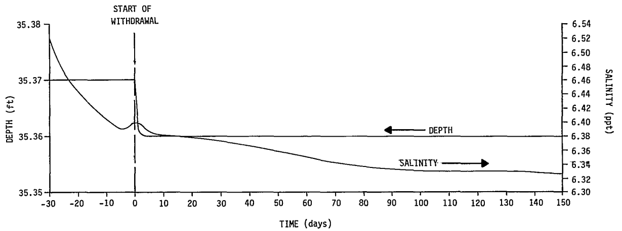
Figure D.13-1. Temporal Variations of Depth and Salinity of Calcasieu Ship Channel
