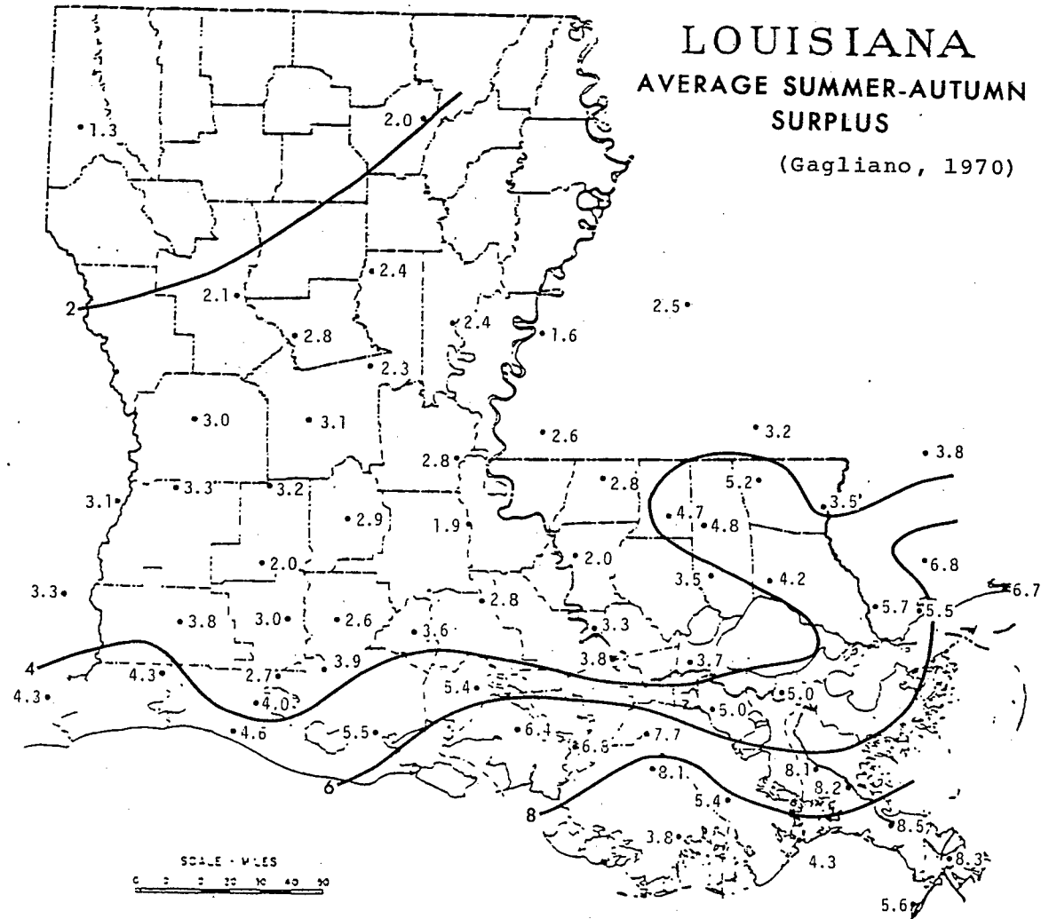
Figure D.1-2. Distribution of average summer-autumn precipitation surplus in south and central Louisiana. Station averages were determined from monthly water balances for the 24-year period between 1945 and 1968. Surplus values are given in inches.
