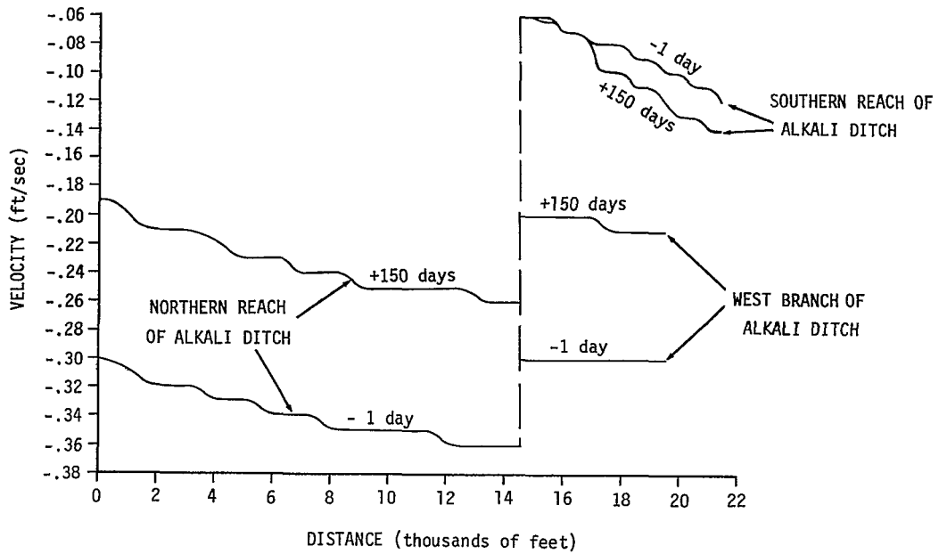
Figure D.12-5. Spatial Variation of Flow Velocity in Alkali Ditch (Without Wind-Driven Tidal Effects)
