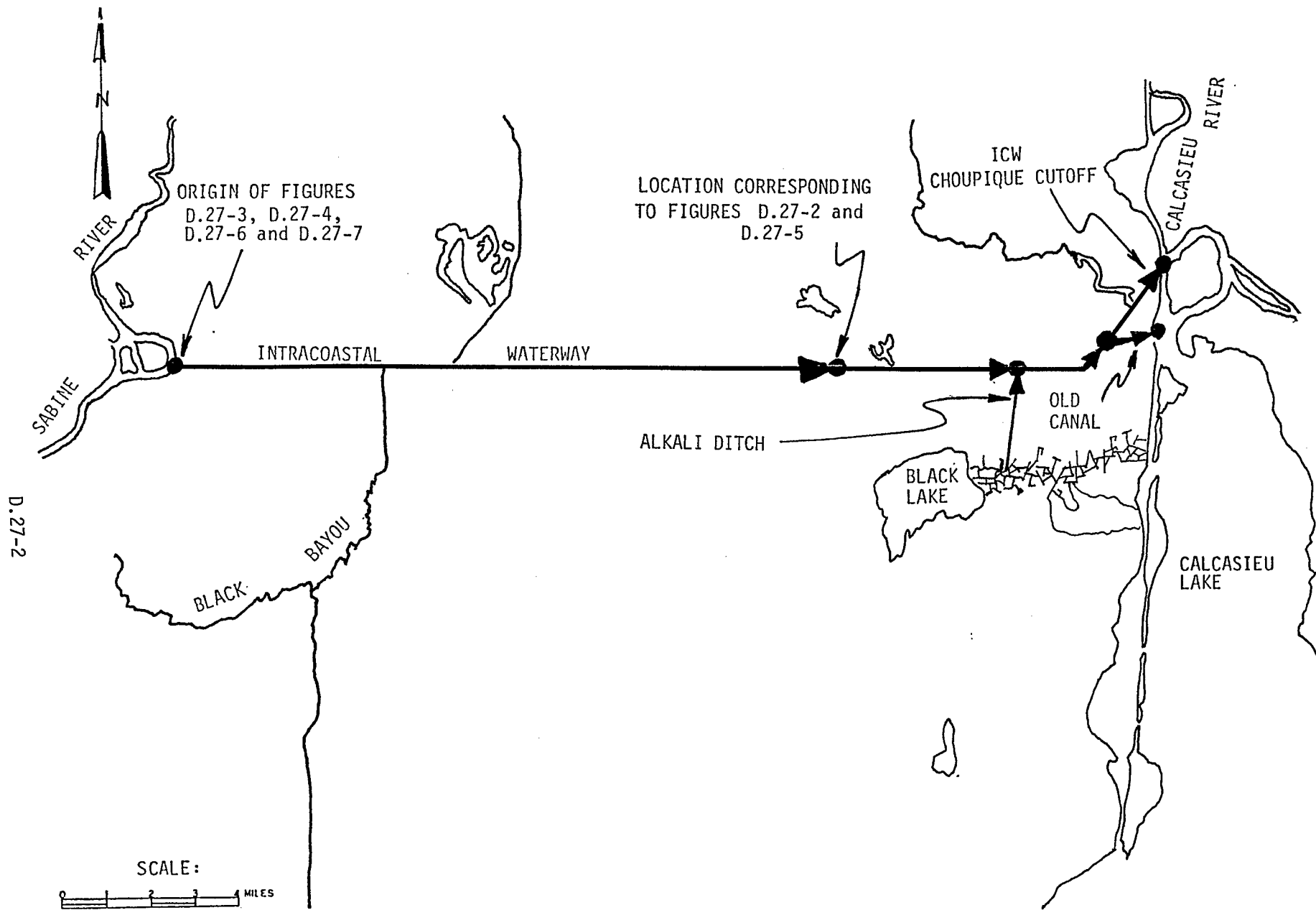
Figure D.27-1. Location of Reference Points and Reaches in the Intracoastal Waterway Network Analysis
