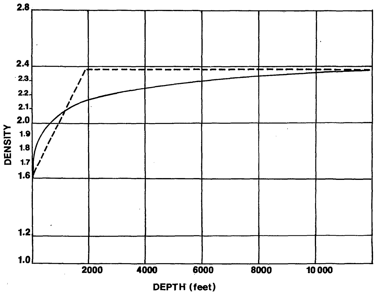
Figure B.2-2 Density of Gulf Coast Shales versus depth of burial
