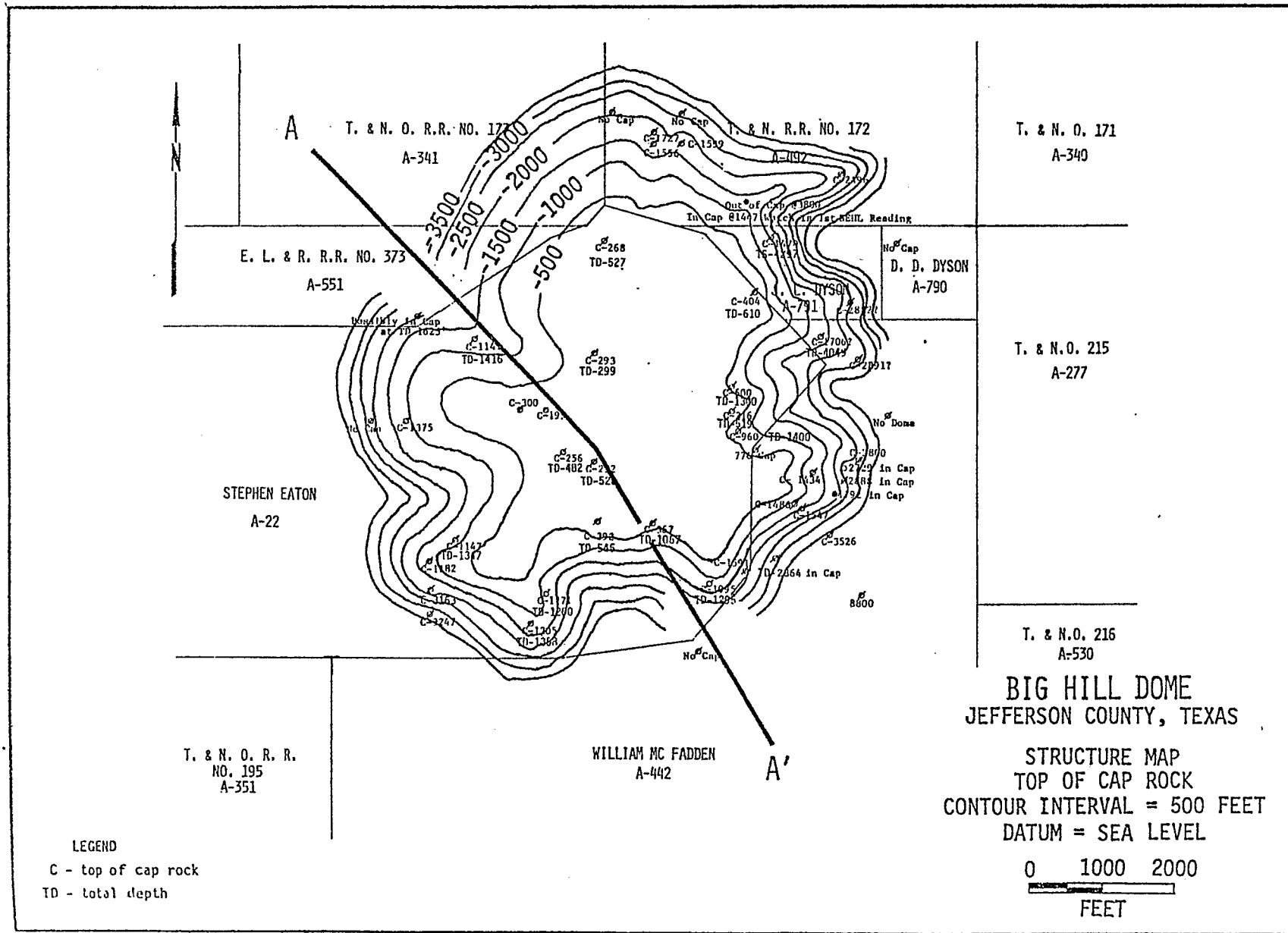
Figure B.3-39 Structure Map - Top of Cap Rock - Big Hill Dome
