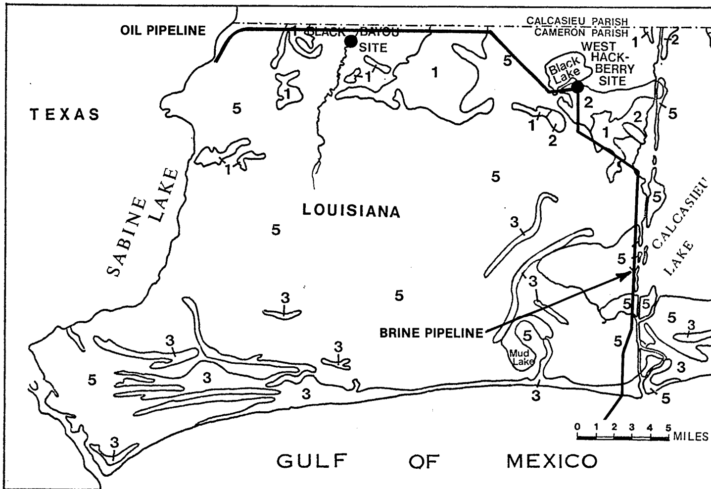
Figure B.3-20 SOIL DISTRIBUTION MAP FOR WESTERN CAMERON PARISH, LOUISIANA IN THE VICINITY OF BLACK BAYOU
