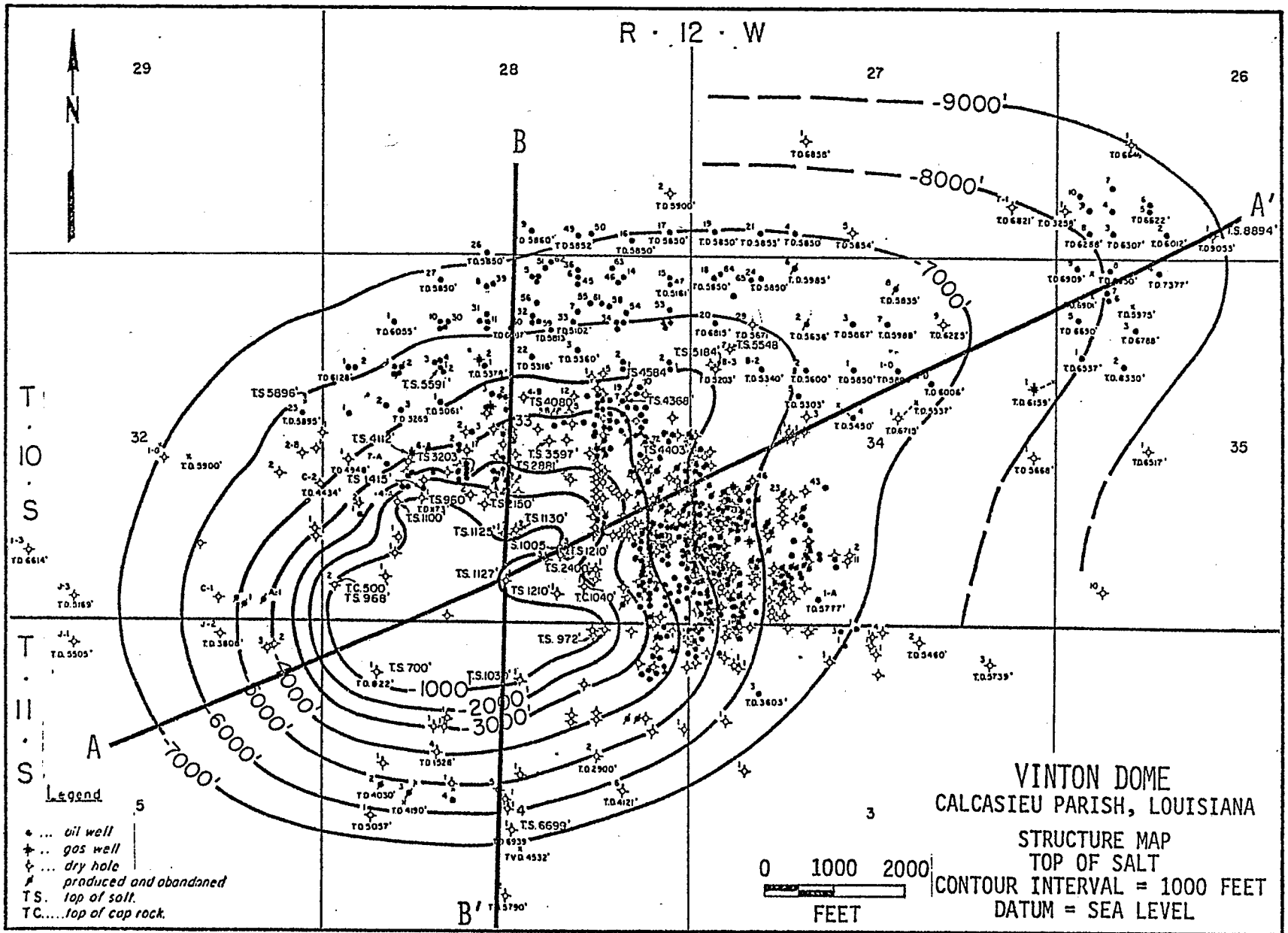
Figure B.3-24 Structure Map - Top of Salt - Vinton Dome
