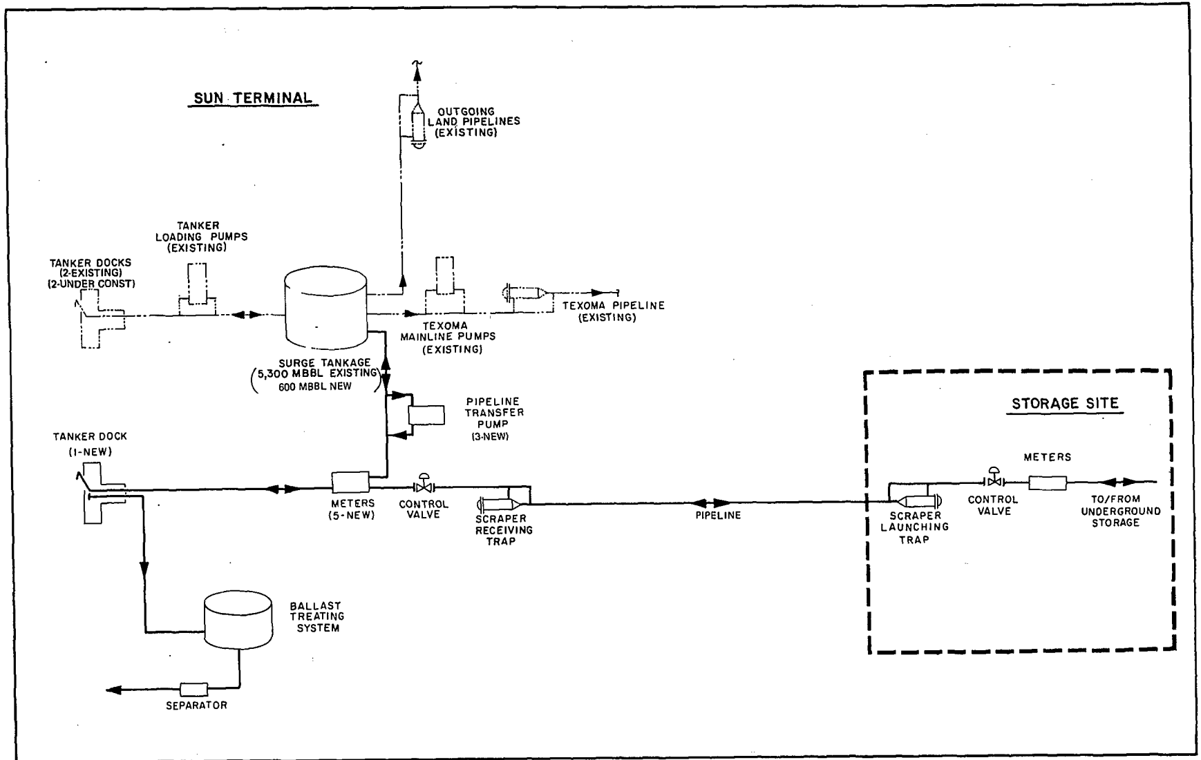
Figure A.4-12 DISTRIBUTION SYSTEM FLOW DIAGRAM
