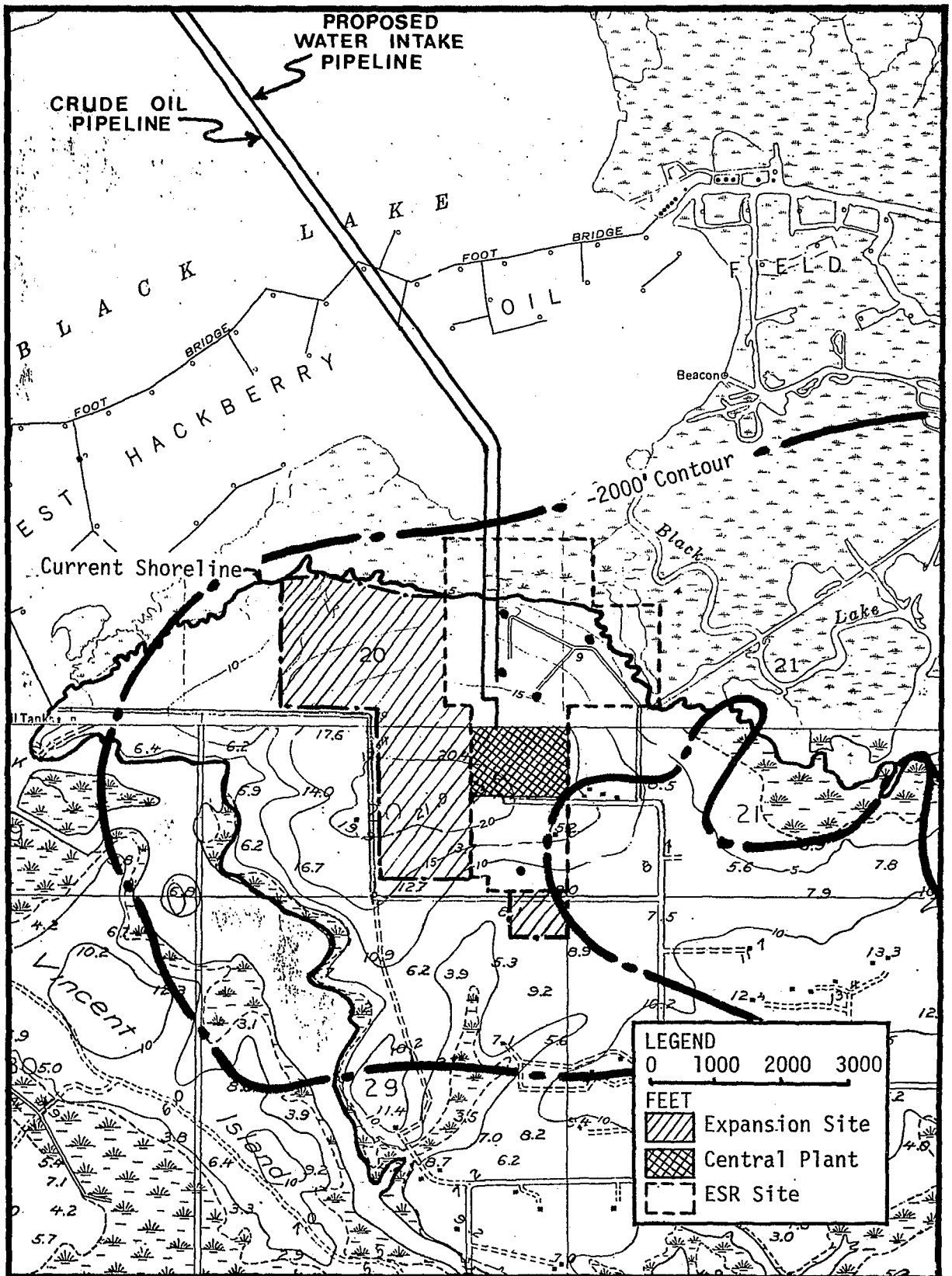
Figure A.4-3 Site Development Plan - West Hackberry
