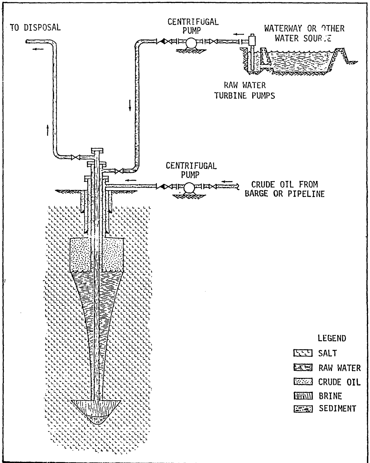
Figure A.3-1 Typical Solution Cavities in Salt Formations
