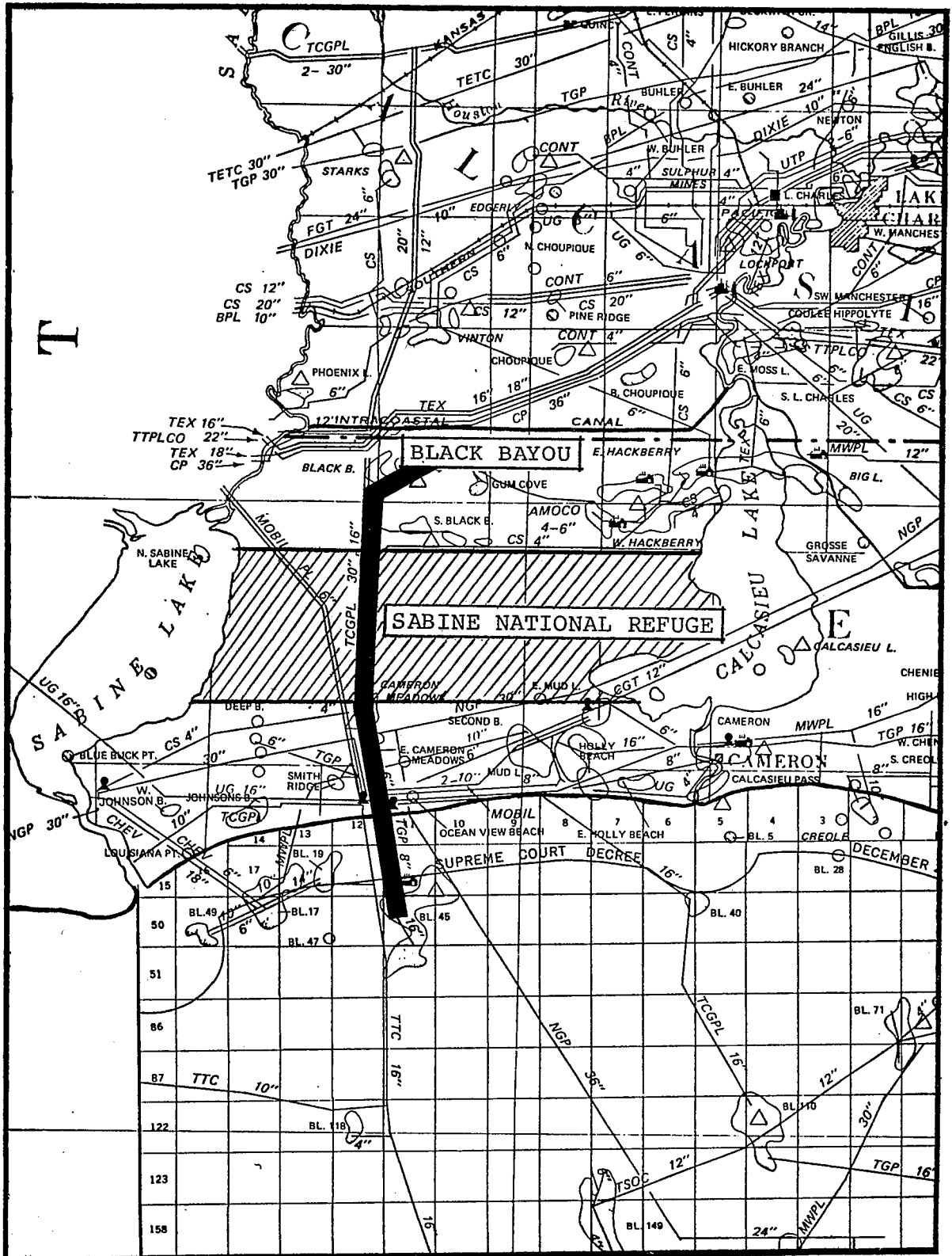
Figure A.5-7 Brine Disposal Pipeline Route
