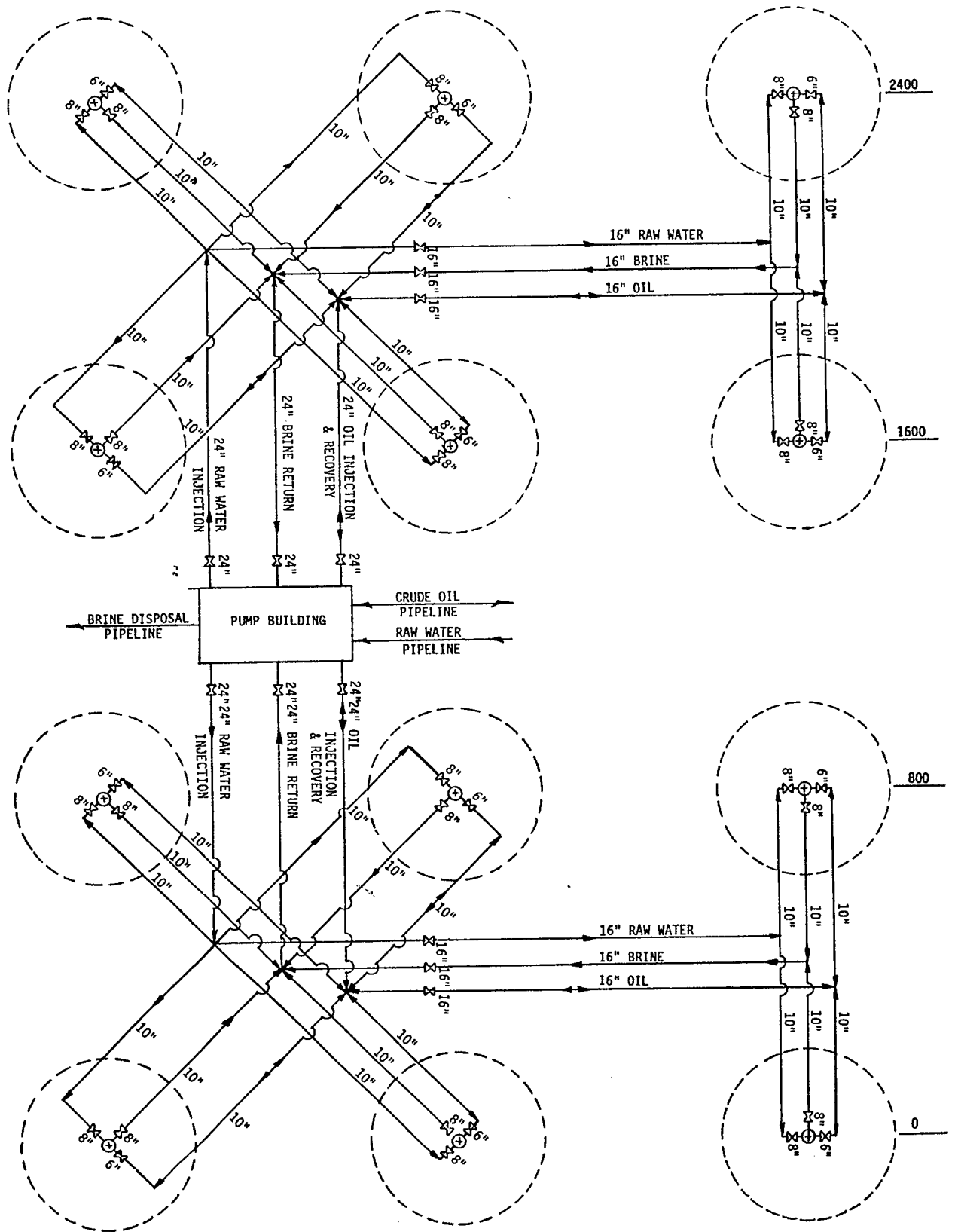
Figure A.7-4 Pipeline Flow Diagram
