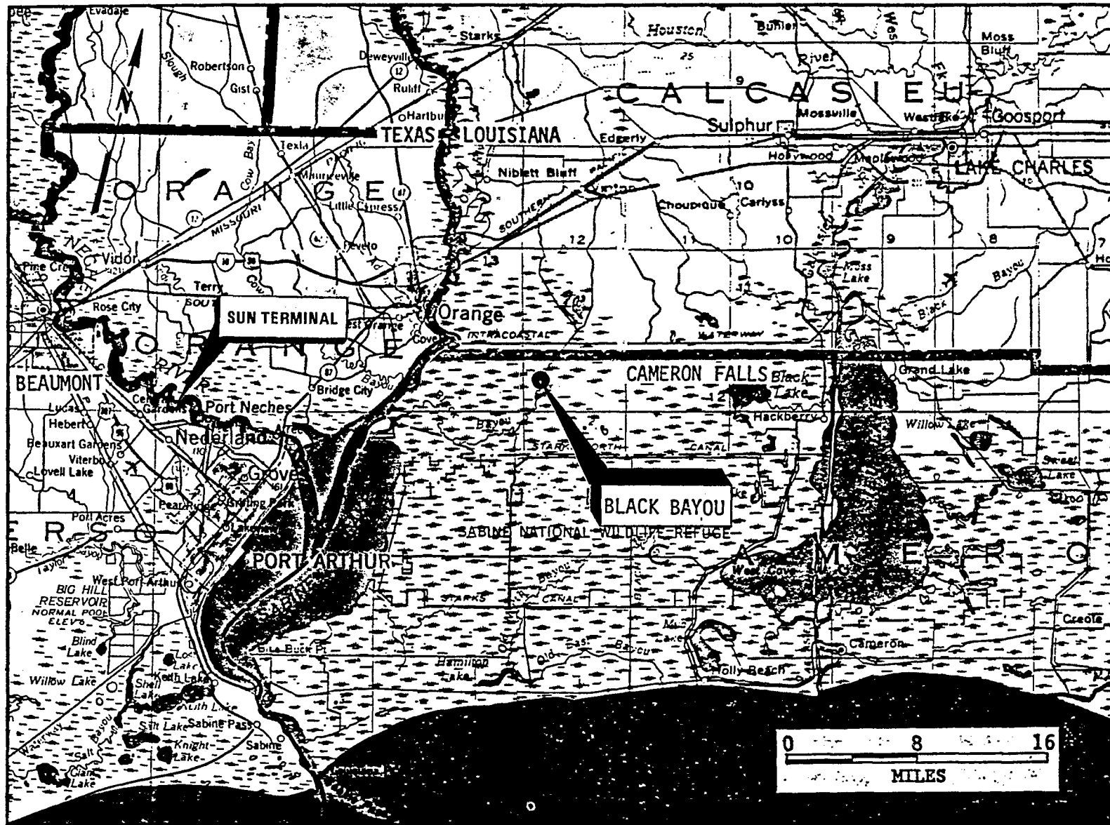
Figure A.5-1 Location Map - Black Bayou Dome
