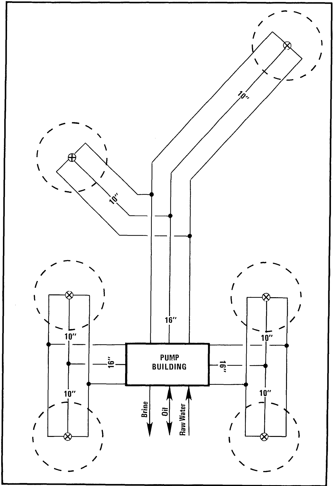
Figure A.6-5 Pipeline Flow Diagram
