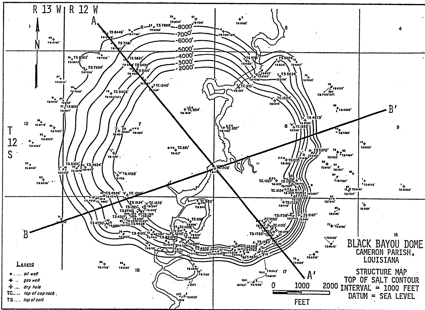
Figure B.3-21 Structure Map - Top of Salt - Black Bayou Dome
