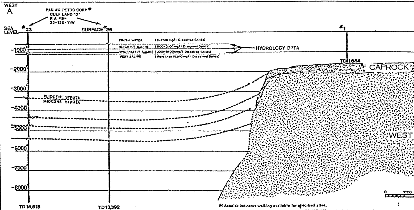
Figure B.3-4. Geological East/West Cross Section West Hackberry Dome A-A'
