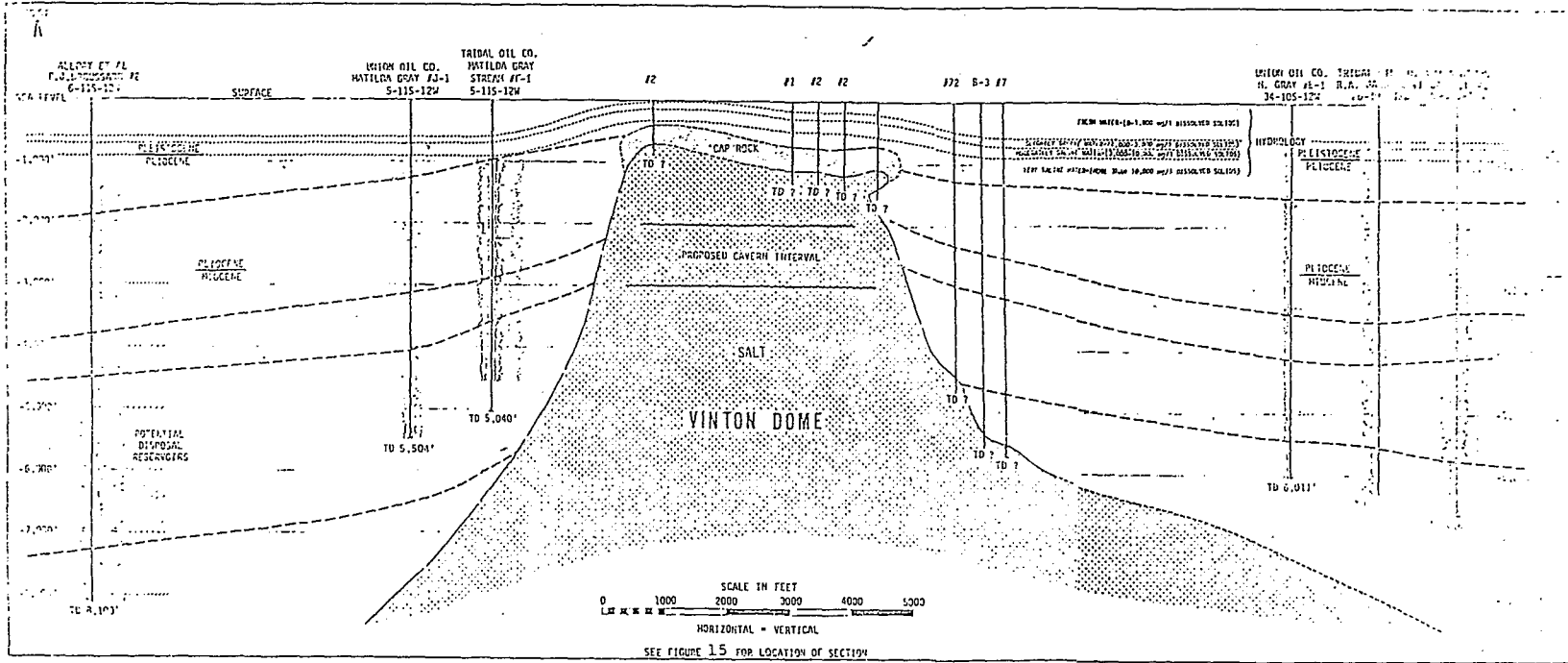
Figure B.3-26 Geologic Cross-Section of Vinton Dome A-A'
