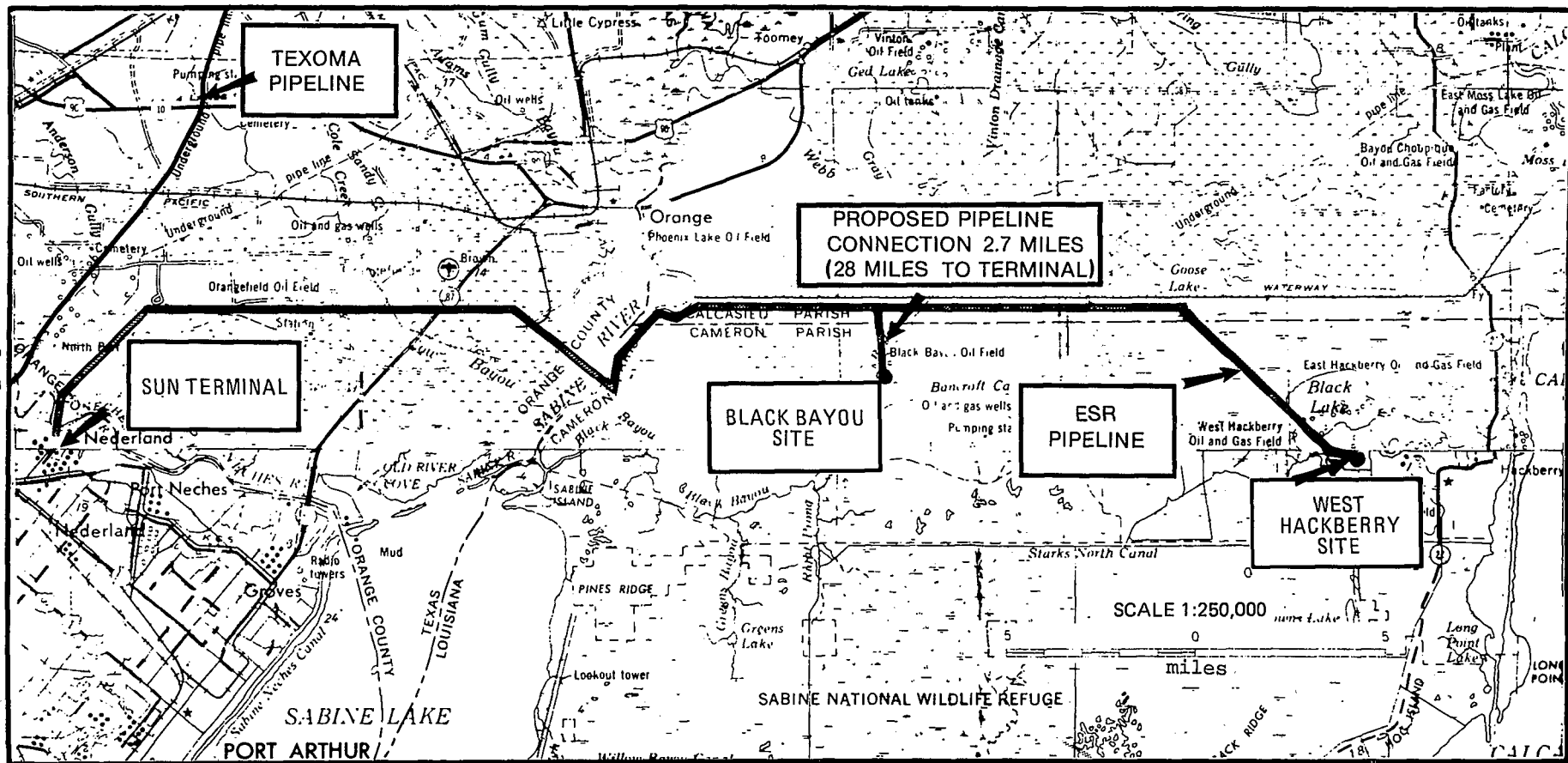
Figure A.5-3 Oil Distribution Pipeline Route
