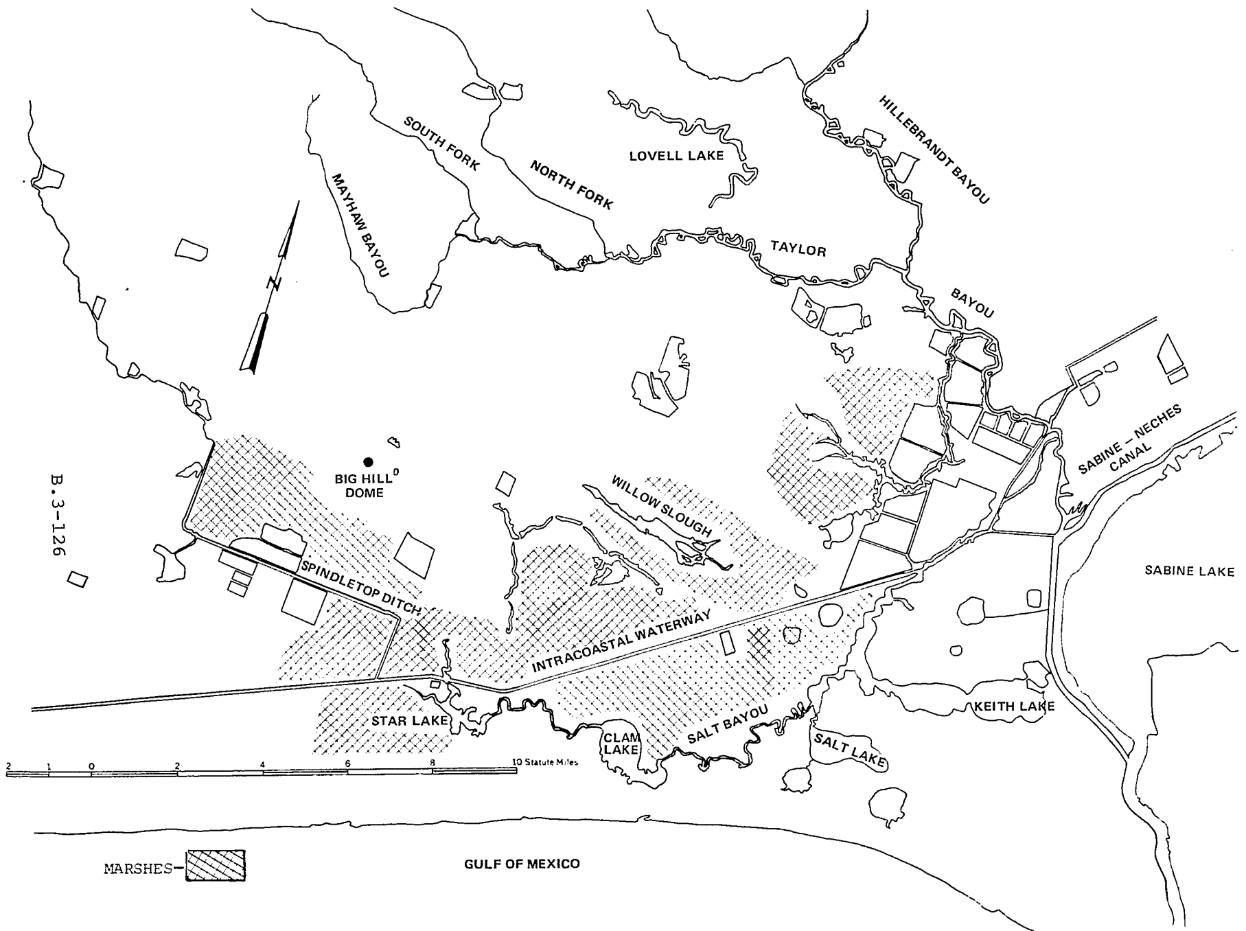
Figure B.3-41 Big Hill Surface Water System
