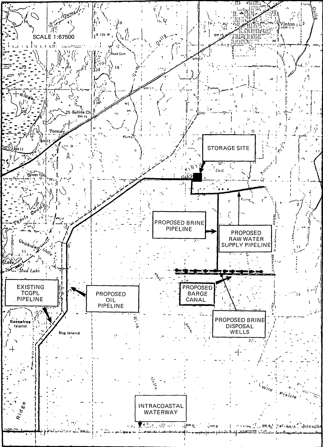
Figure A.6-3 Systems Components Layout
