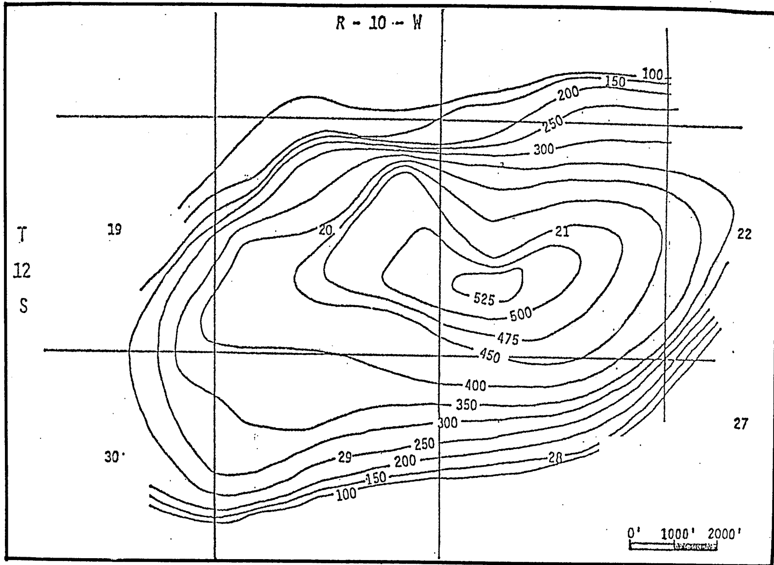
Figure B.3-3. Isopach Map of Thickness of Caprock West Hackberry, Cameron Parish, La.
