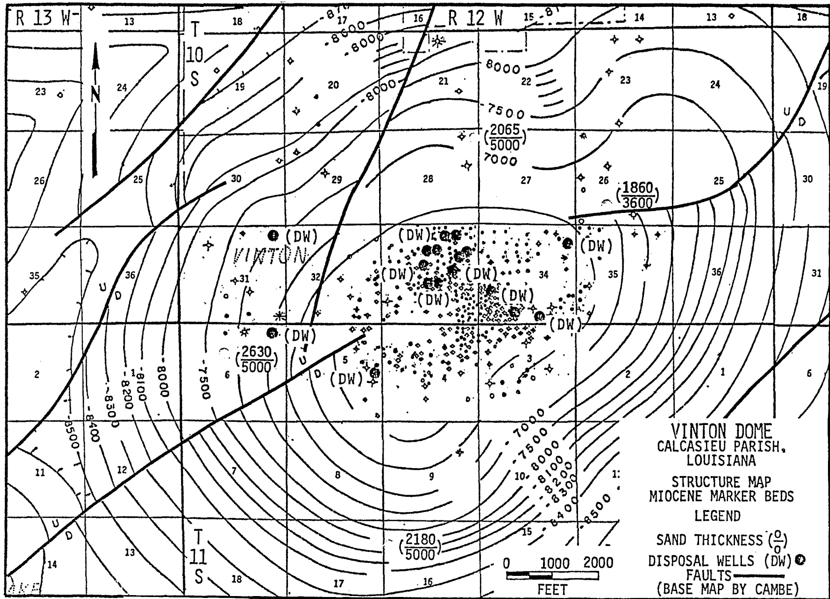
Figure B.3-27 Structure Map, Miocene Marker Beds - Vinton Dome
