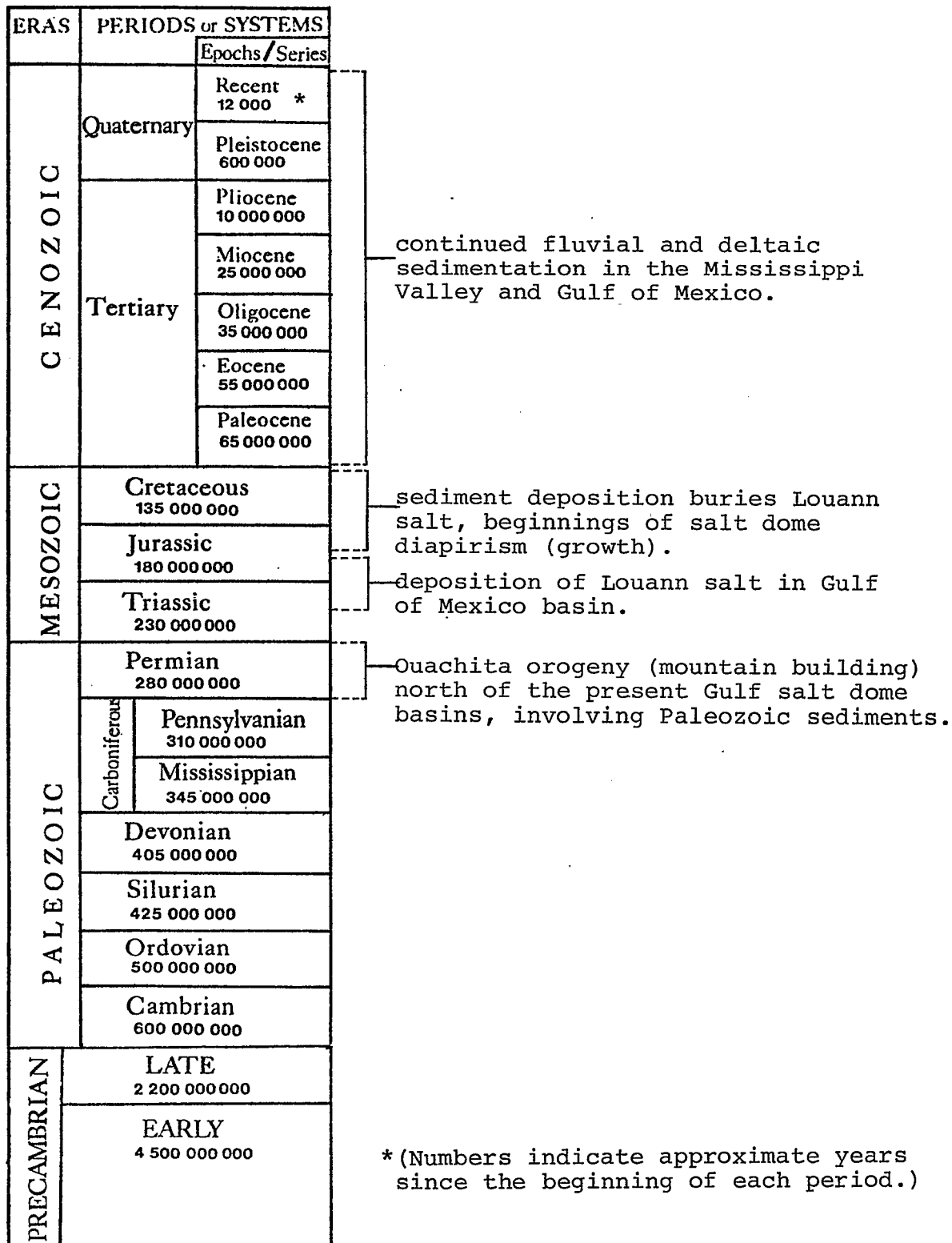
Figure B.2-1 Geologic Time Scale
