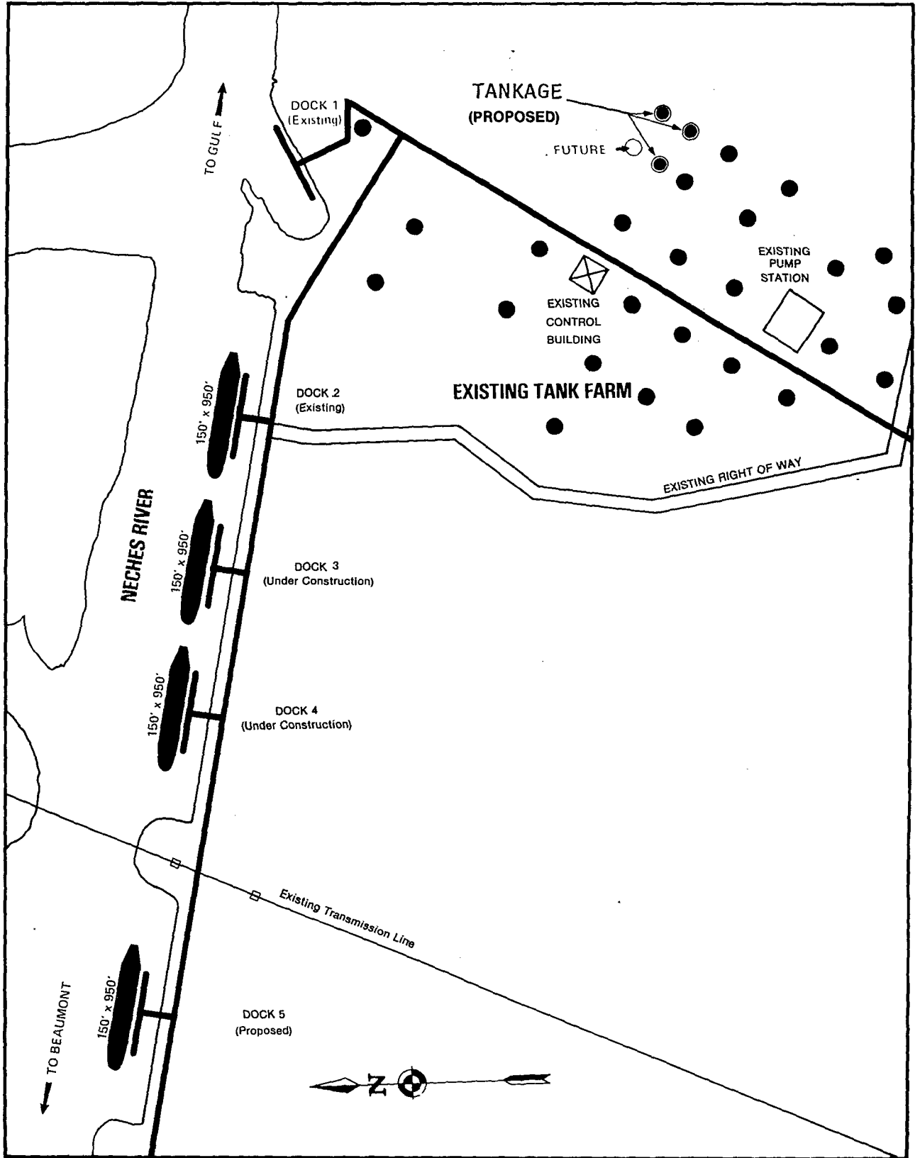
Figure A.4- 11 Sun Terminal Site Plan
